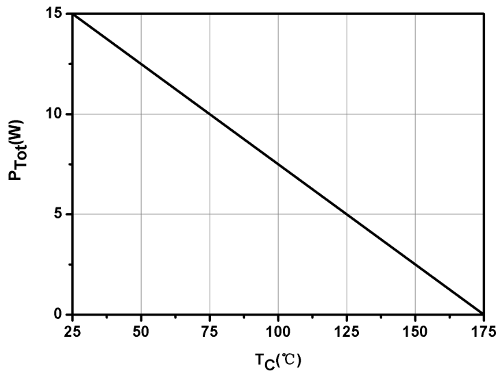
Fig.6-Power Derating
