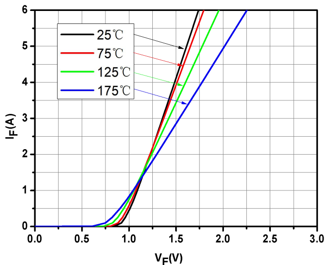
Fig.1-Typical Forward Voltage
